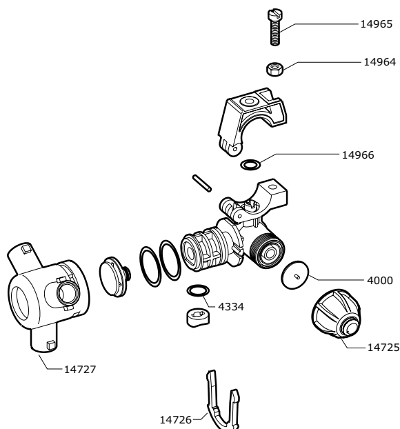
PICO TRIJET COMPACTO 1-4 VUELTA D 1-2 - 10 (COD. 4176)
