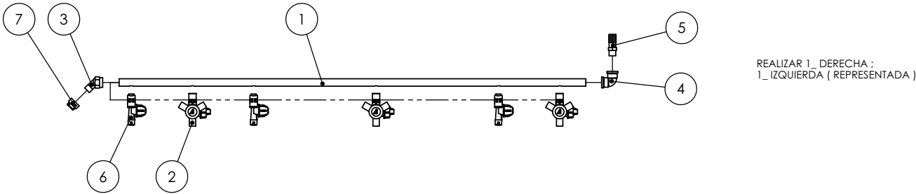
LINEA ALA MAYOR EXT - 25/28 - .35/.525 (cod. 9167)
