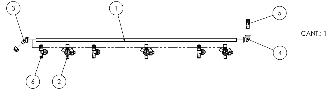
LINEA ALA MAYOR EXT - 25/28 - .35/.525 (cod. 9167)
